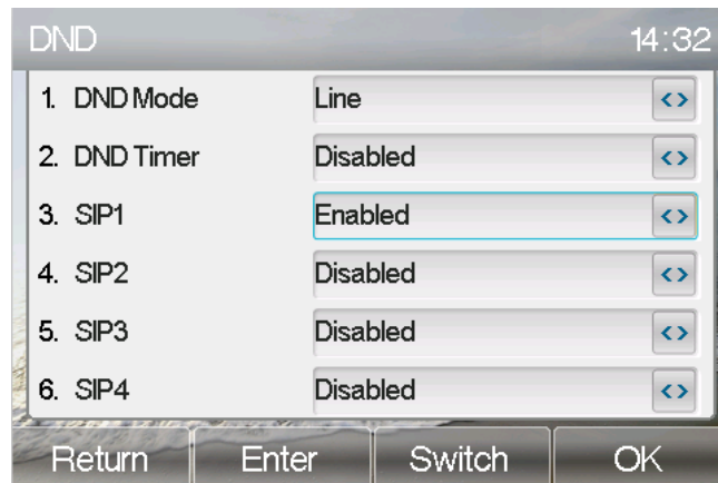
Figure 41 - Configure DND
